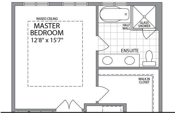
PART. UPPER LEVEL W/ OPT. ENSUITE - ELEV. A
