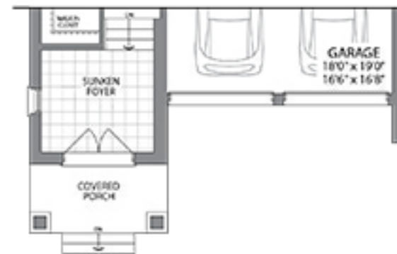
PARTIAL MAIN LEVEL - ELEV. C
