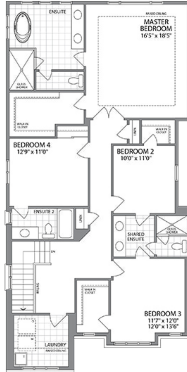
UPPER LEVEL - ELEV. A
