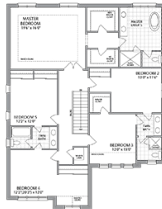
OPT. UPPER LEVEL WITH 5 BEDROOMS ELEV. B
