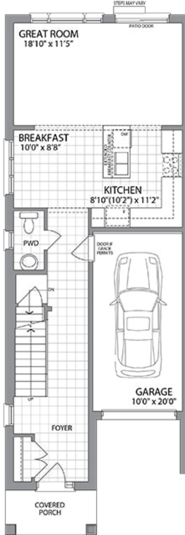
MAIN LEVEL - ELEV. A
