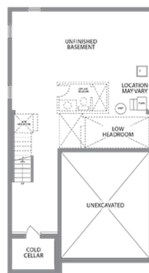
LOWER LEVEL ELEVATION B & C
