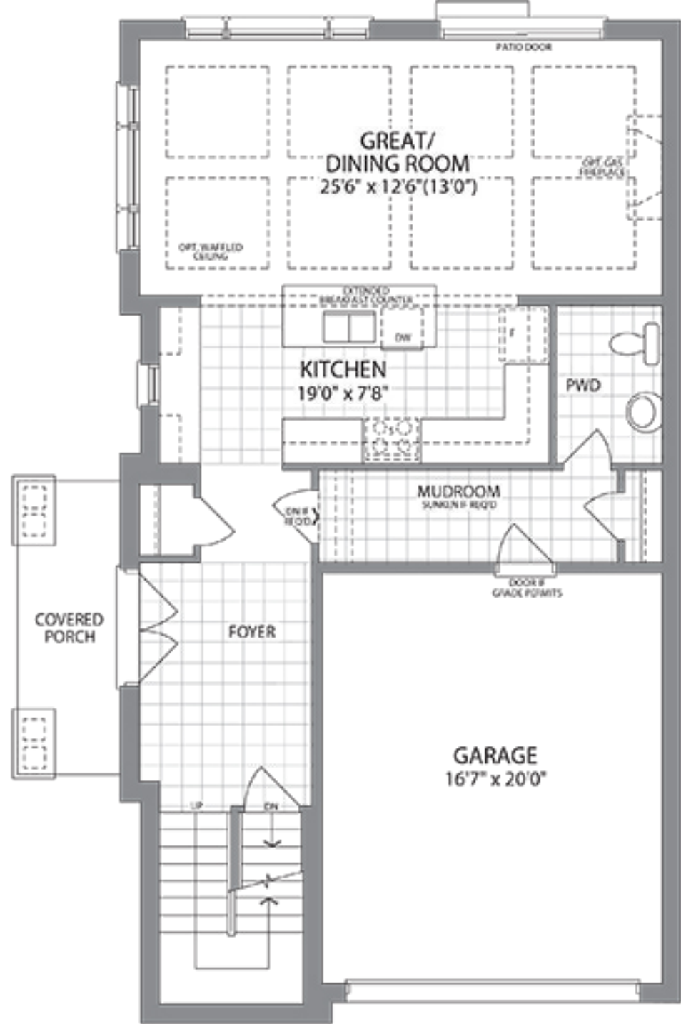
MAIN LEVEL ELEVATION B
