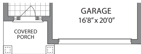
PARTIAL MAIN LEVEL ELEVATION C
