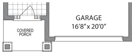
PARTIAL MAIN LEVEL ELEVATION A
