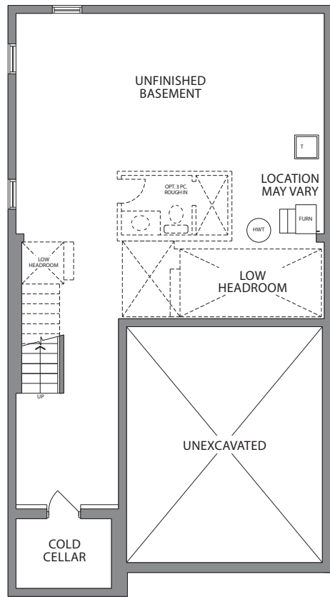
LOWER LEVEL ELEVATION A, B, & C
