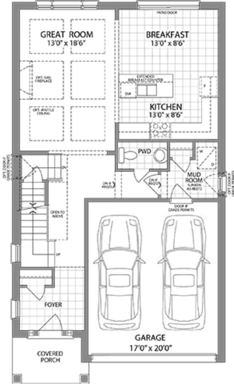
MAIN LEVEL ELEVATION A & B
