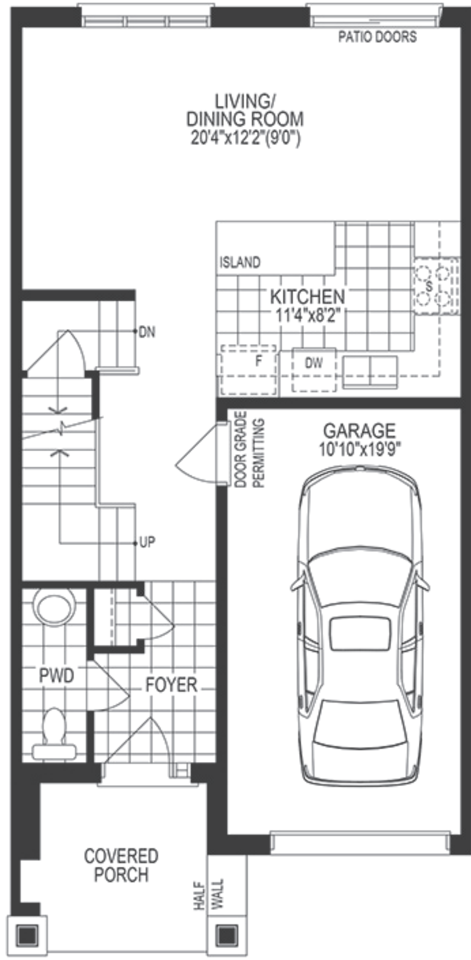
MAIN LEVEL ELEV. A
