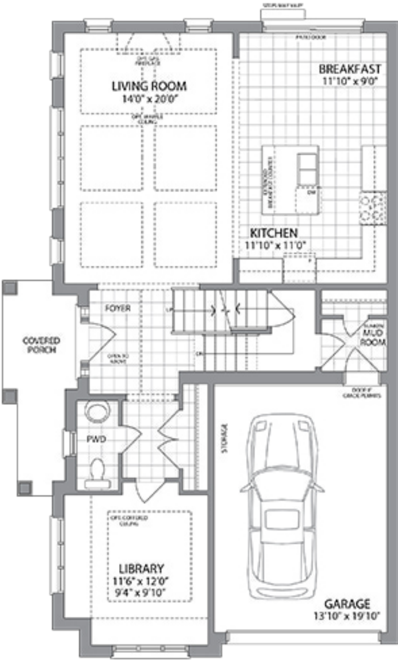
MAIN LEVEL - ELEV. A
