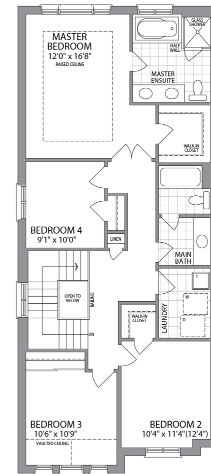
UPPER LEVEL - ELEV. B
