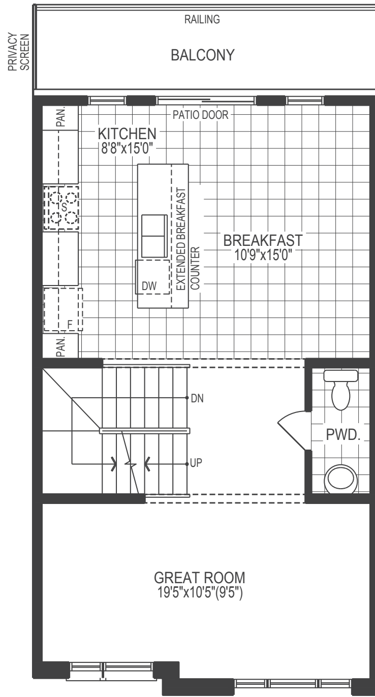
MAIN LEVEL ELEV. B
