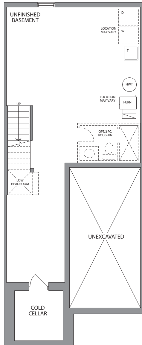
LOWER LEVEL ELEV. A
