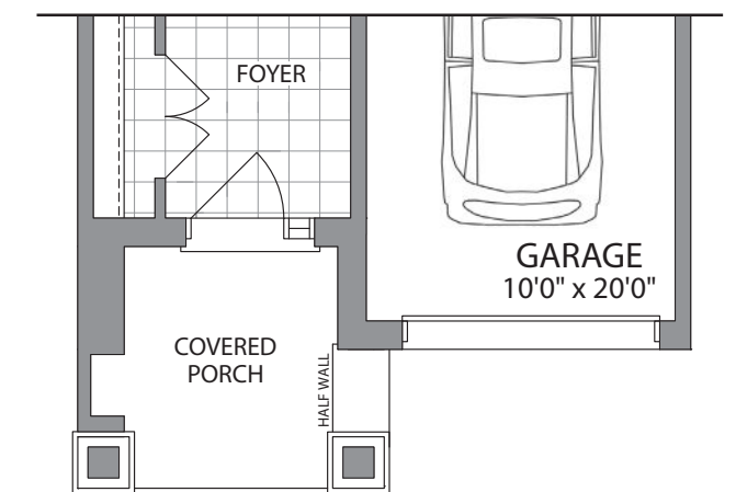
PART. MAIN LEVEL ELEV. B
