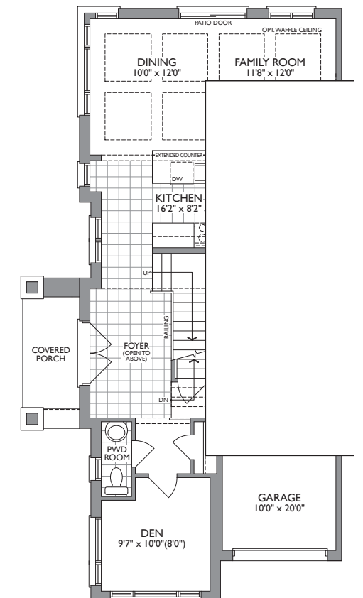
PARTIAL MAIN FLOOR ELEV. B
