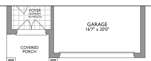
PARTIAL MAIN LEVEL ELEV. B & C
