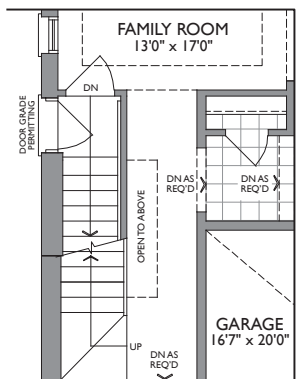
PARTIAL MAIN LEVEL WITH OPT. SIDE DOOR (LOCATION MAY VARY BASED ON GRADE) ELEV. A, B & C
