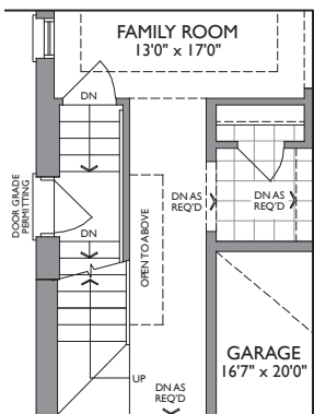
PARTIAL MAIN LEVEL WITH OPT. SIDE DOOR (LOCATION MAY VARY BASED ON GRADE) ELEV. A, B & C
