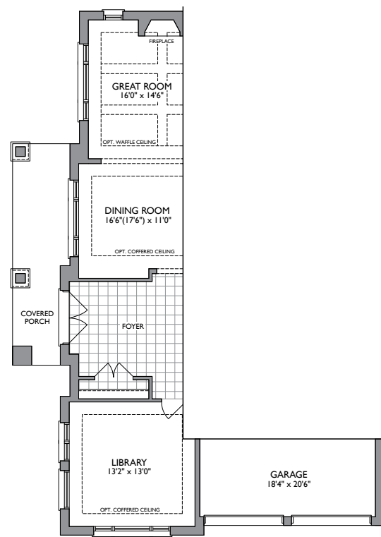
PARTIAL MAIN FLOOR ELEV. B
