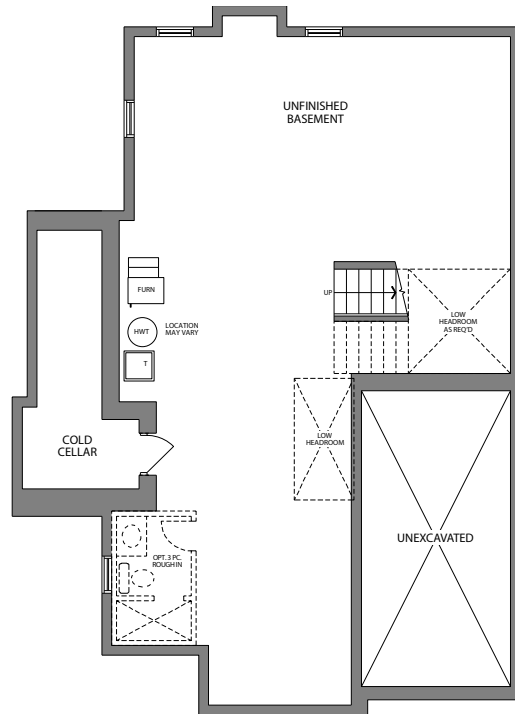
LOWER LEVEL - ELEV. A & B
