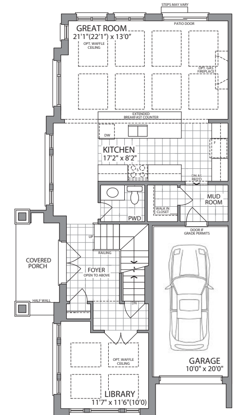
MAIN LEVEL - ELEV. B
