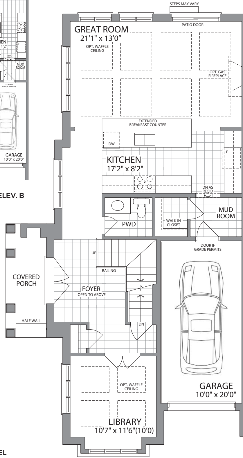
MAIN LEVEL - ELEV. A
