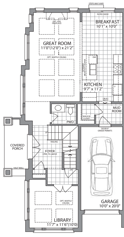
ALT. MAIN LEVEL - ELEV. B
