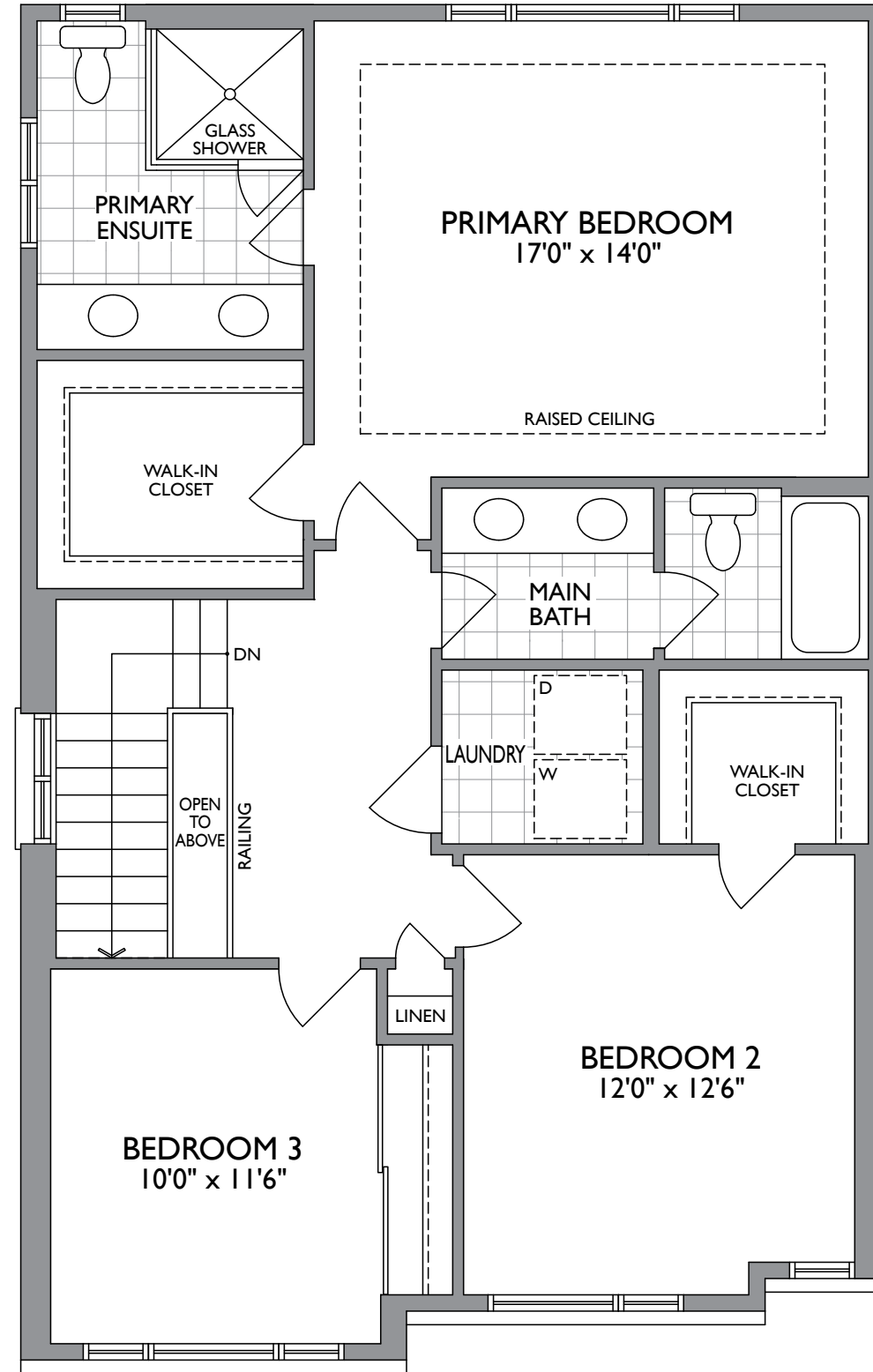
UPPER LEVEL ELEV. A
