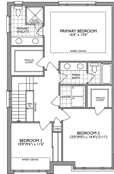
UPPER LEVEL ELEV. B
