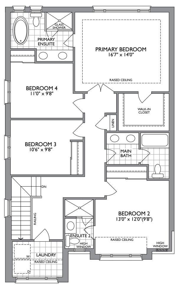
UPPER LEVEL ELEV. B
