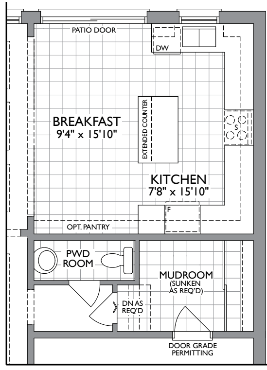
PARTIAL ALT. MAIN LEVEL ELEV. A, B & C
