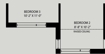
ELEVATION B1 (EXPOSED END) PARTIAL UPPER LEVEL
