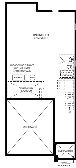
ELEVATION A & B | LOWER LEVEL
