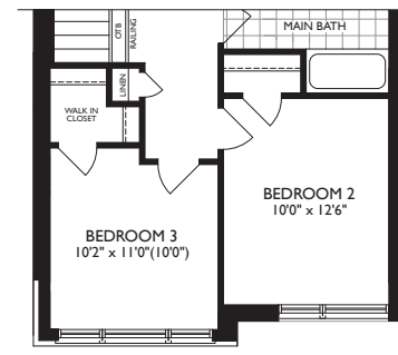
PART. UPPER LEVEL - ELEV. C
