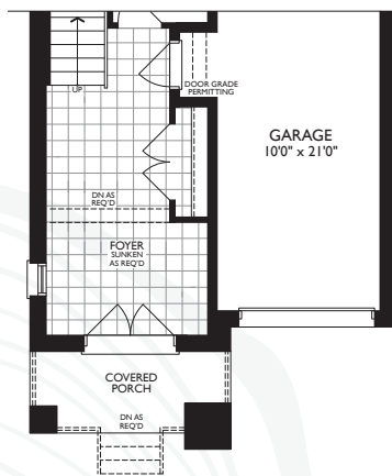
PART. GROUND LEVEL - ELEV. C PART. GROUND LEVEL - ELEV. B
