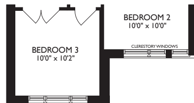
PART. UPPER LEVEL - ELEV. C
