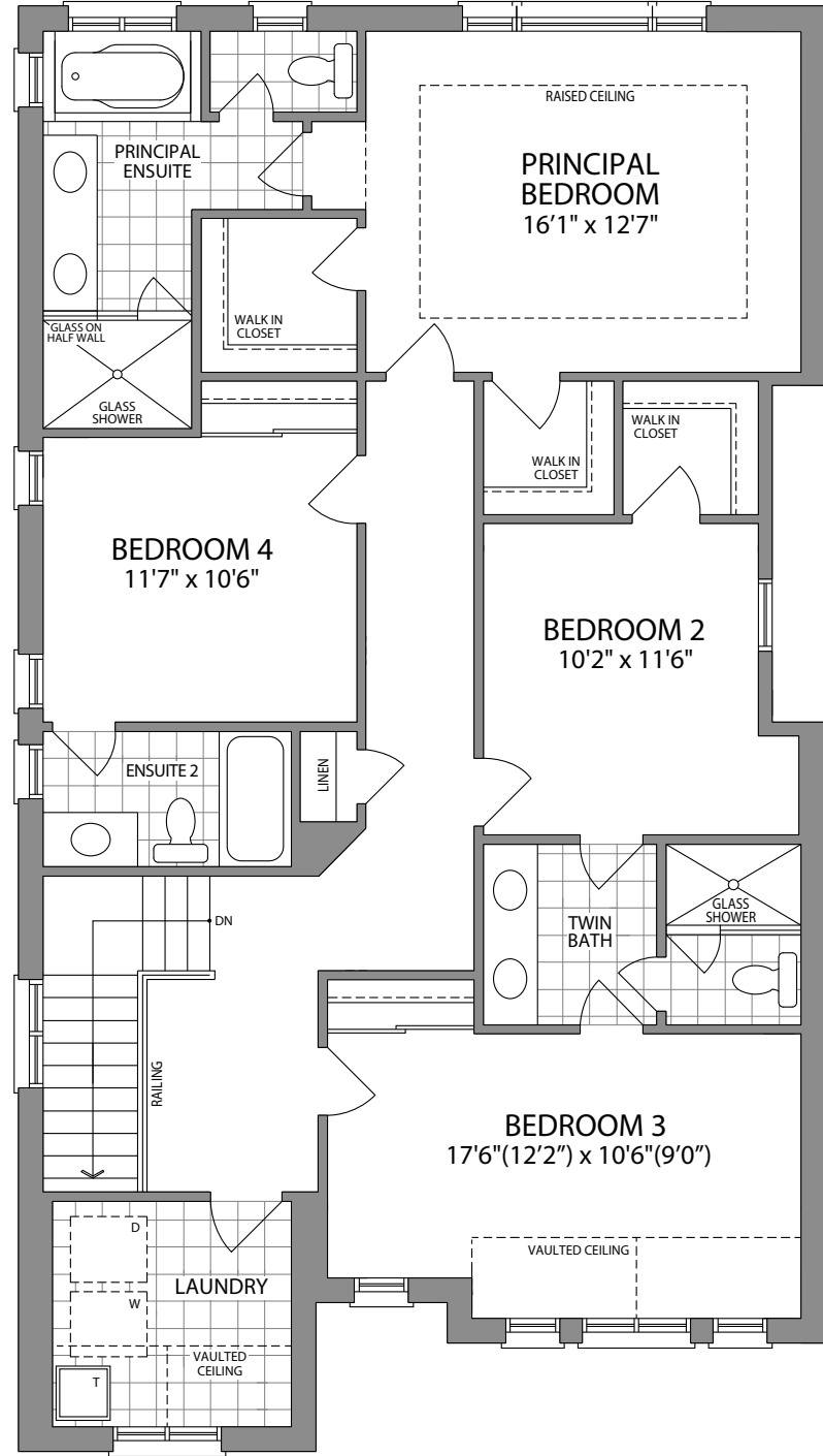
UPPER LEVEL ELEVATION C
