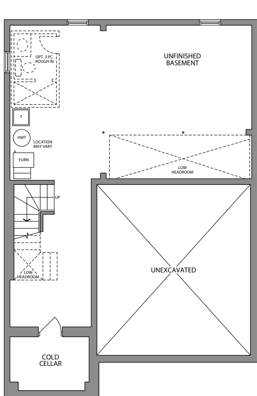
LOWER LEVEL ELEVATION A
