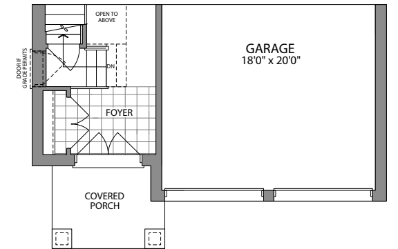
PARTIAL MAIN LEVEL ELEVATION B & C
