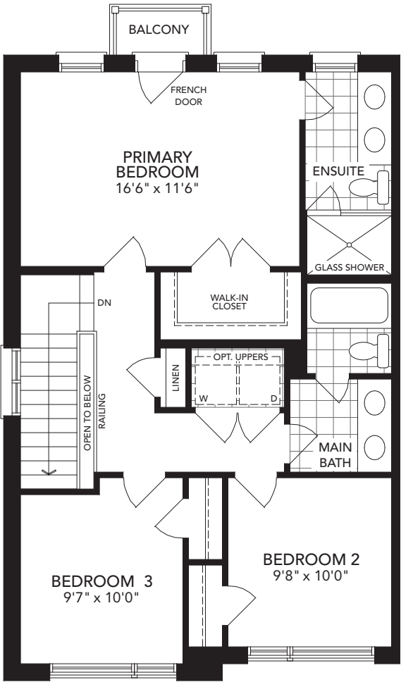
Upper Level ELEV. A
