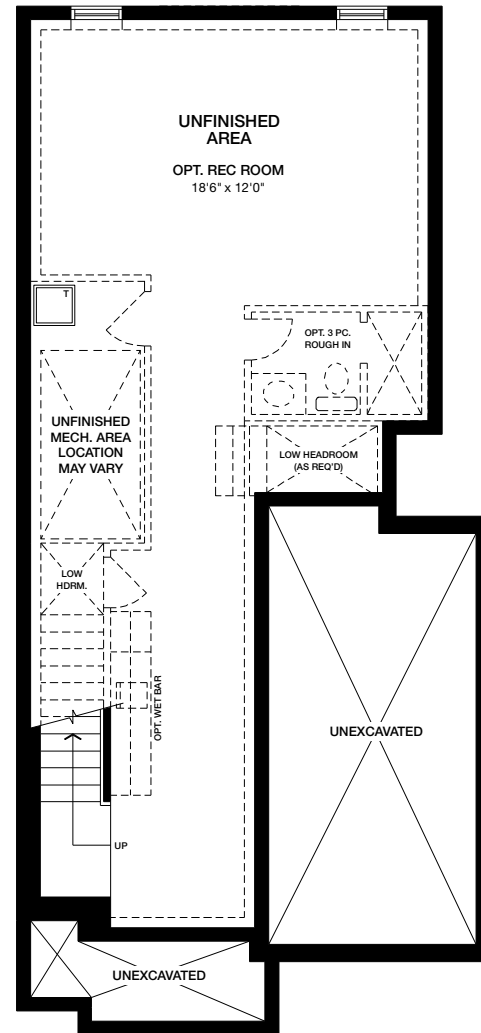
Lower Level ELEVATION A
