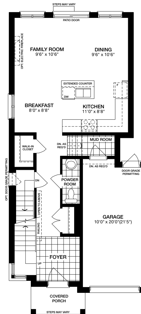
Main Level ELEVATION C
