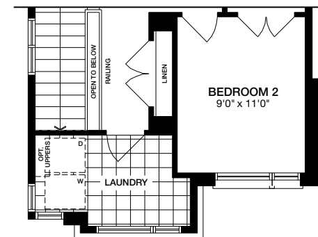
Partial Upper Level ELEVATION C
