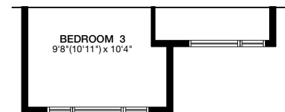
Partial Upper Level ELEVATION C
