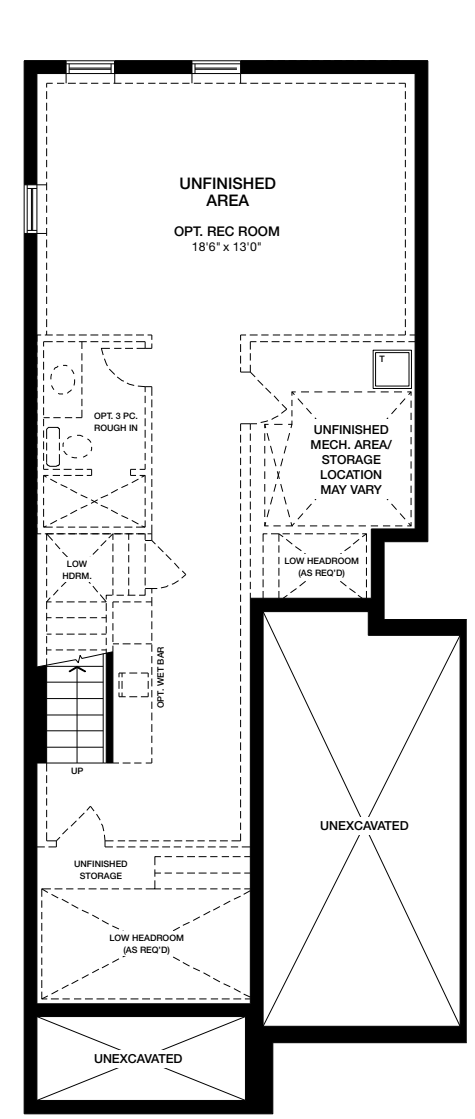
Lower Level ELEVATION A
