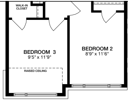
Partial Upper Level ELEVATION C
