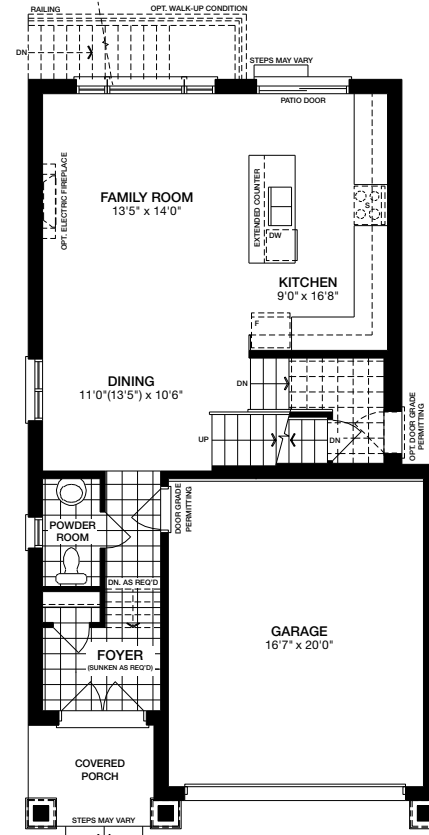
Main Level ELEVATION B
