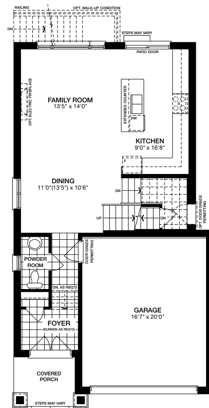
Main Level ELEVATION C
