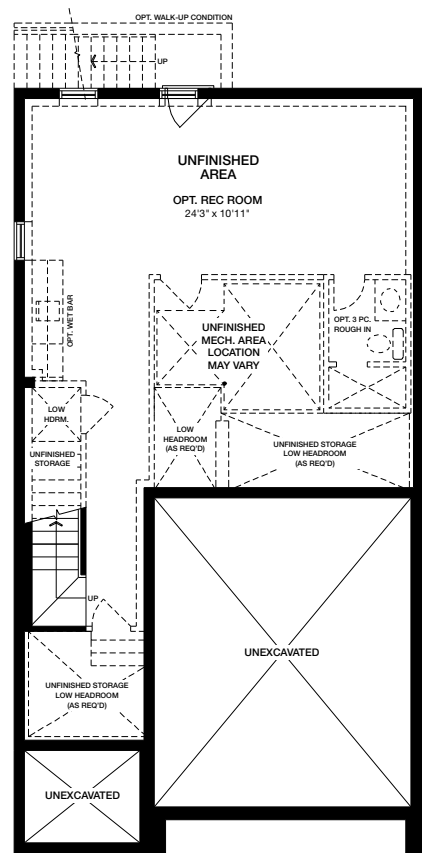
Lower Level ELEVATION A
