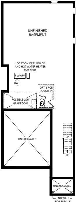
ELEV. A & B | LOWER LEVEL
