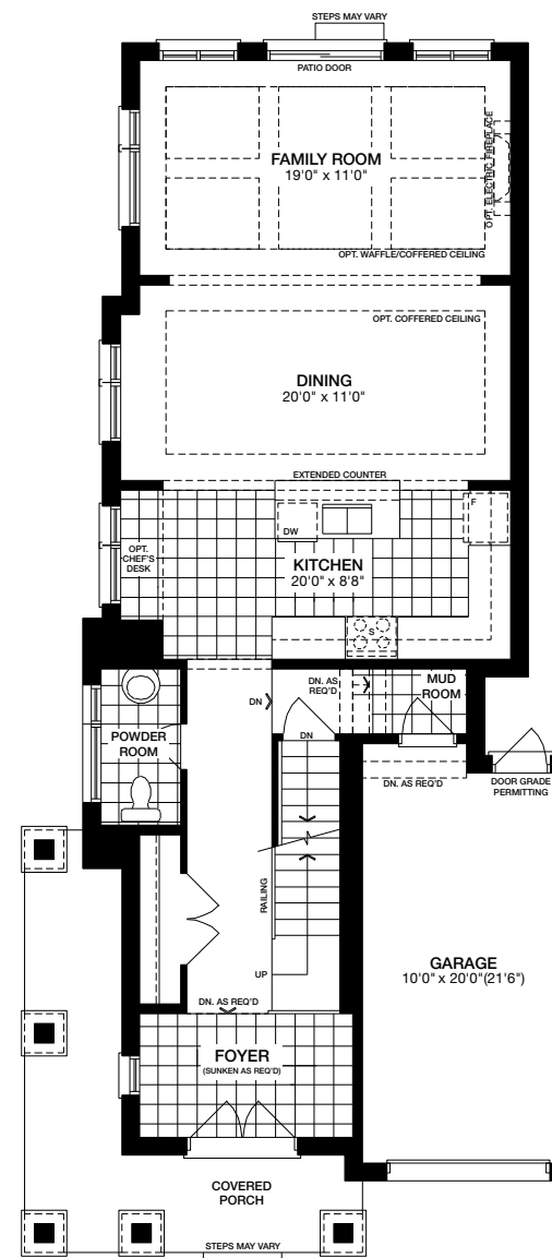
Main Level ELEVATION C
