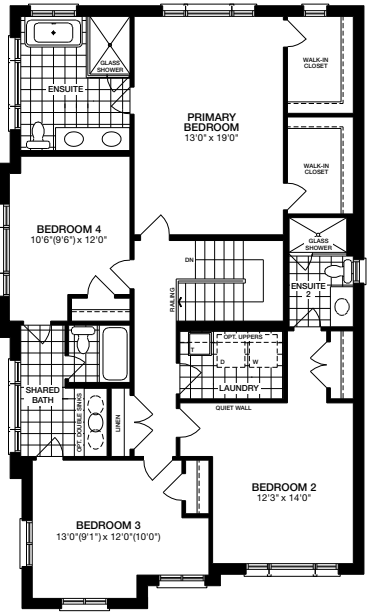
Upper Level ELEVATION B
