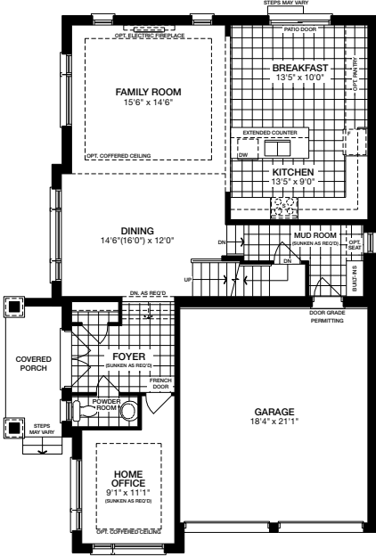
Main Level ELEVATION C
