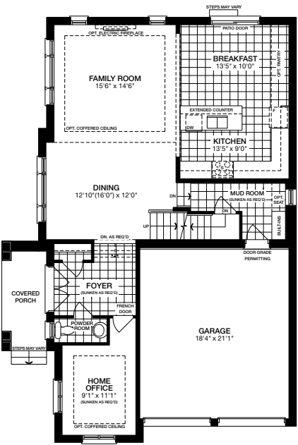
Main Level ELEVATION B
