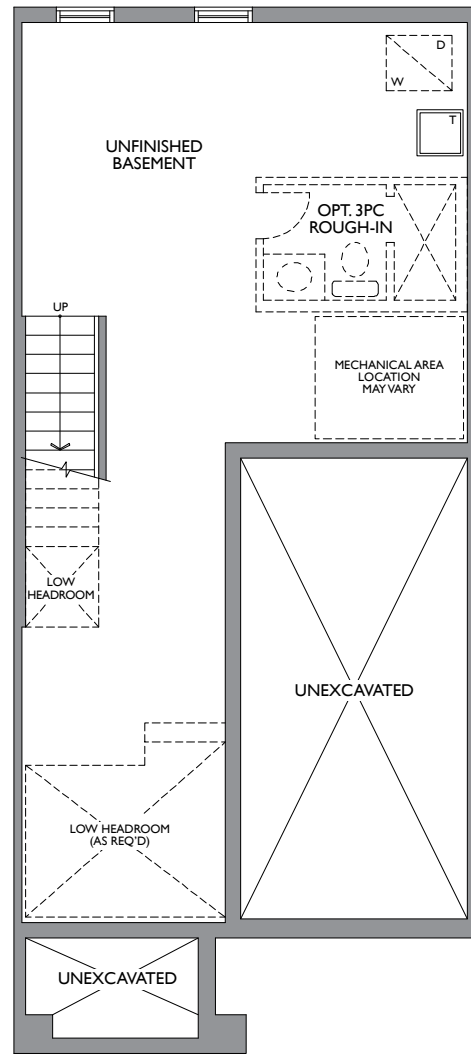
LOWER LEVEL ELEV. A & B
