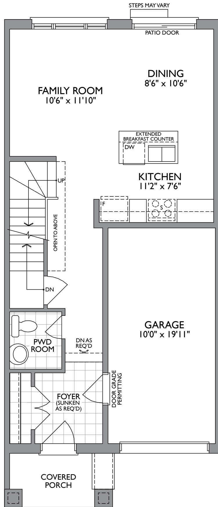
MAIN LEVEL ELEV. A & B
